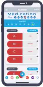
Medication
